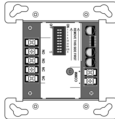
4090-9010 8 A IDNet Relay IAM Package (shown approximately 1/2 size)
